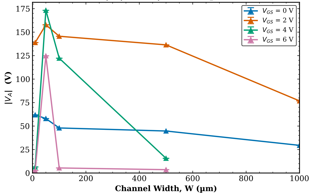
TFT2 Transistor 2 |V_A| vs W | L = 160\text{ }\mu\text{m}
